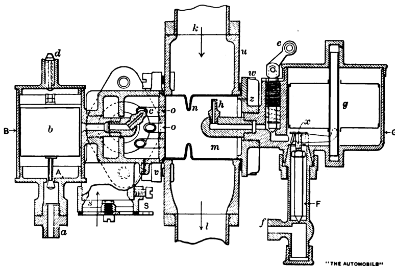
FIG. 2.—VERTICAL SECTION OF CLUDEL CARBURETER FOR HEAVY OILS.
